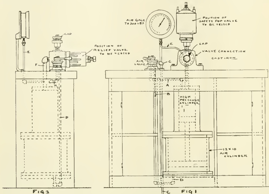
DEVICE FOR TESTING POP AND RELIEF VALVES.
